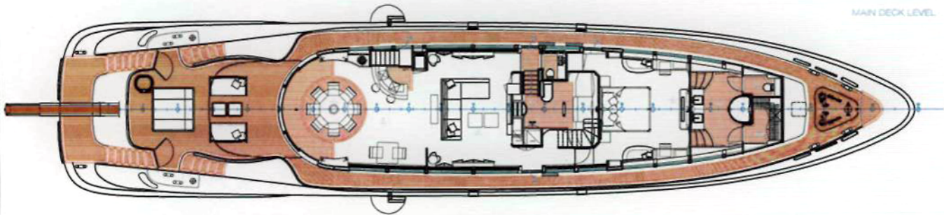
MAIN DECK LEVEL
